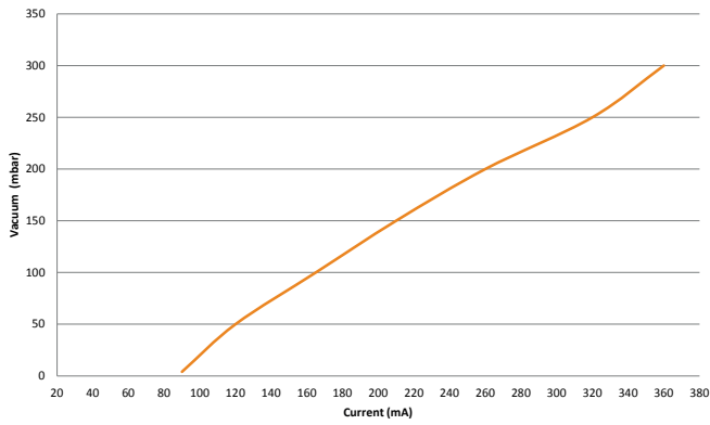
Vacuum Vs. Current (5V DC at maximum freeflow)
