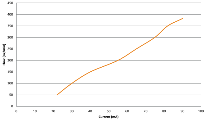
Flow Vs. Current (@ 5V DC)
