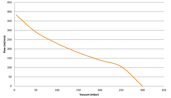
Flow Vs. Vacuum (5V DC)
